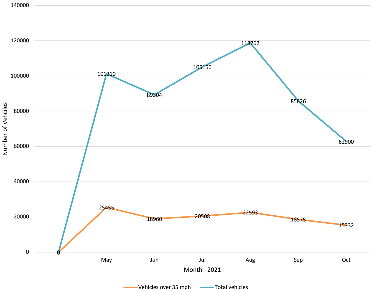
Drift Vehicle Activated Sign (VAS) data. May - Oct 2021
