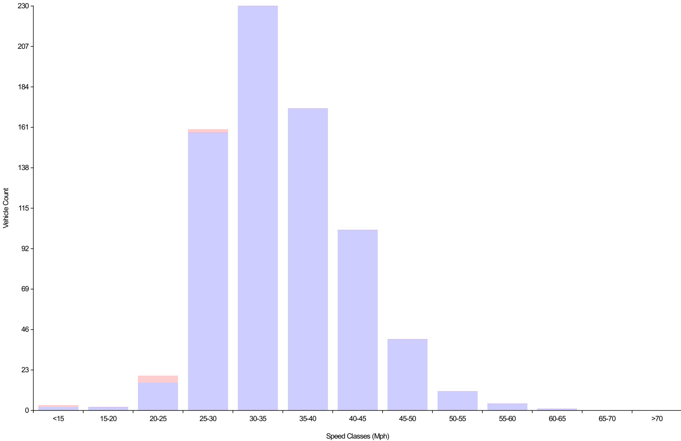
Vehicle Counts By Speed Class Daily Overview for Wed Feb 1 2023
