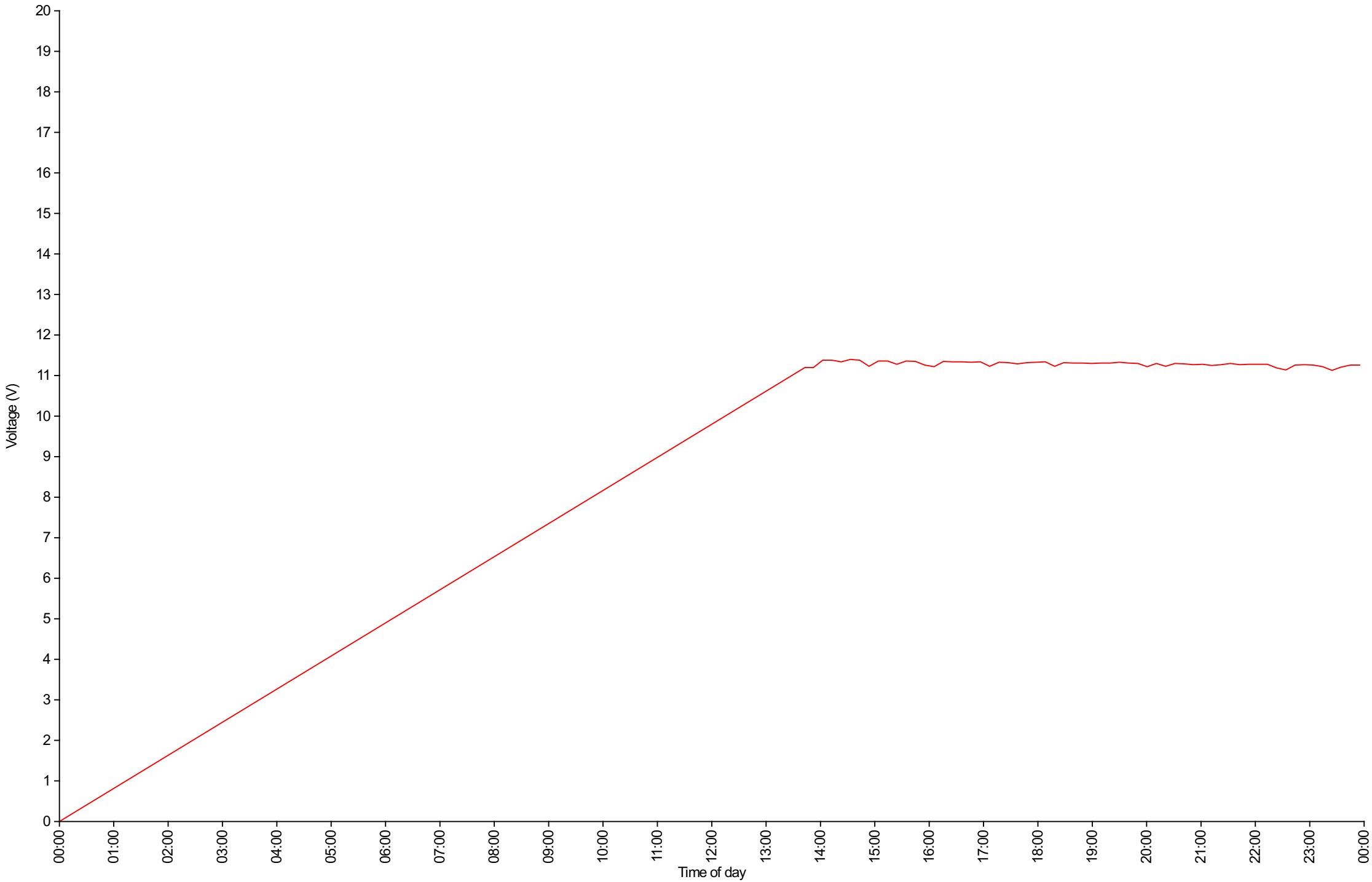
Voltage Daily Overview for Thu Mar 9 2023
