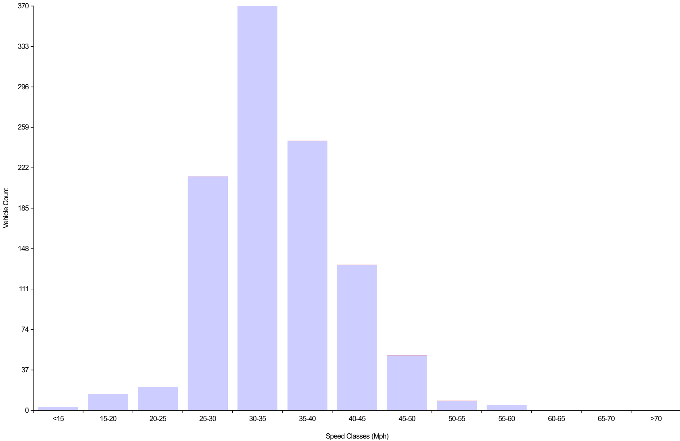
Vehicle Counts By Speed Class Daily Overview for Tue Feb 28 2023
