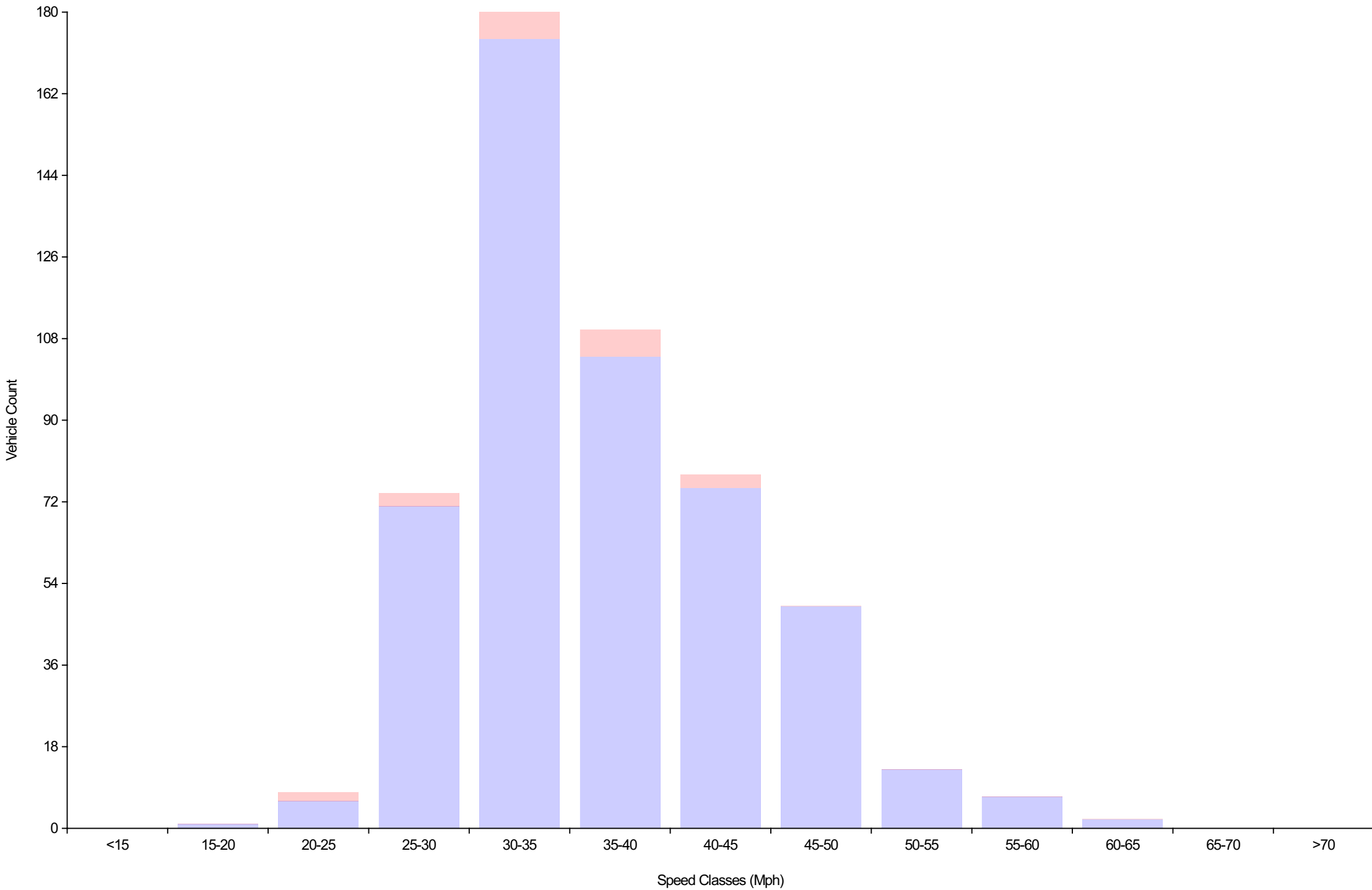
Vehicle Counts By Speed Class Daily Overview for Fri Mar 10 2023
