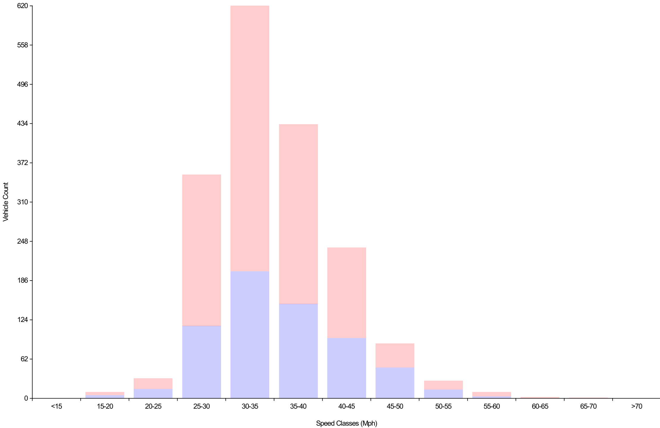
Vehicle Counts By Speed Class Daily Overview for Sun Feb 26 2023
