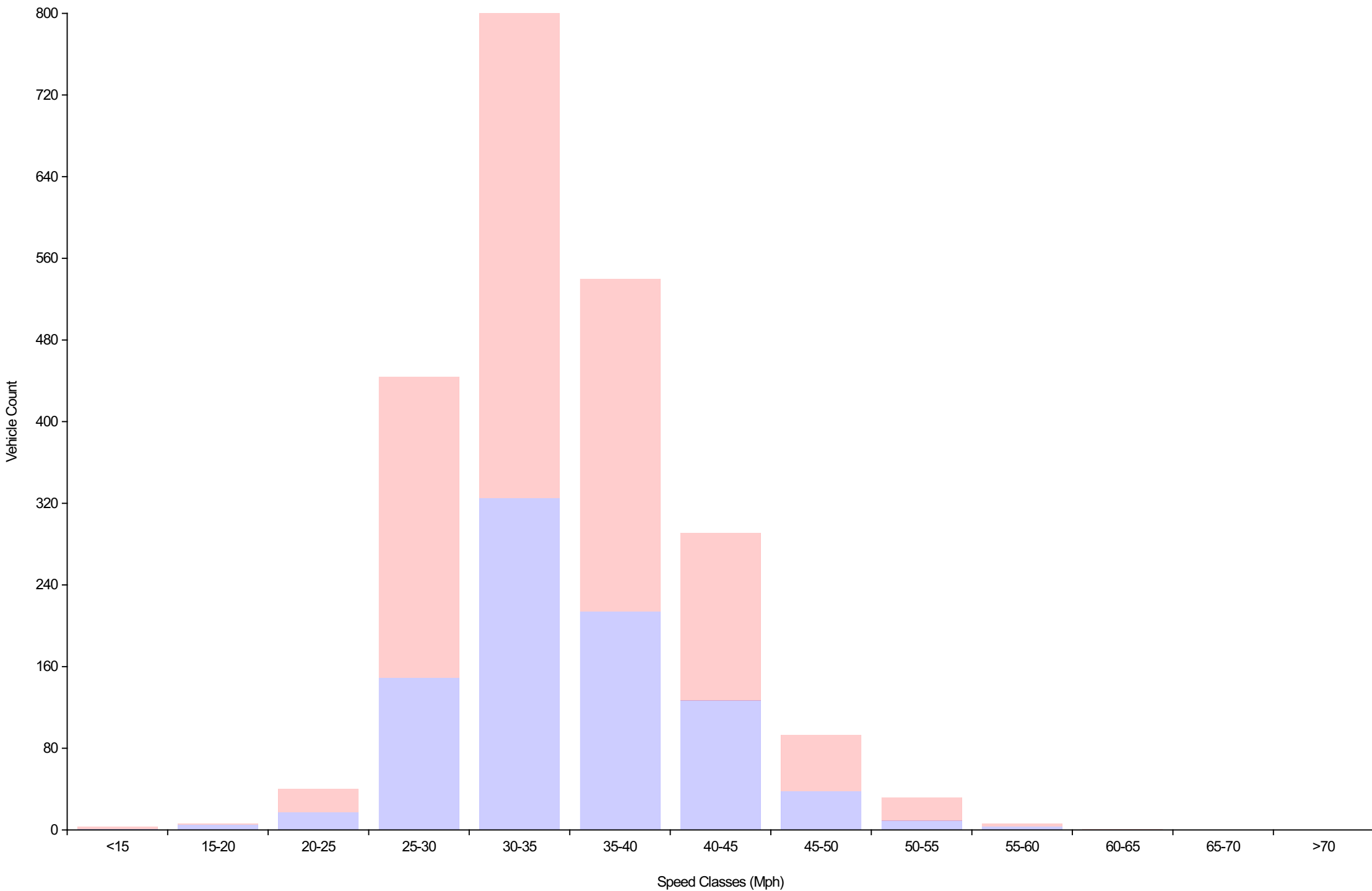
Vehicle Counts By Speed Class Daily Overview for Sat Feb 25 2023
